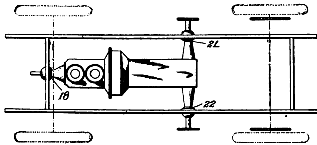
MORGAN THREE-POINT MOTOR AND GEAR BOX SUPPORT.
